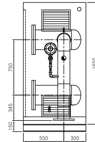
VIEW :A-A' (S=1:1)
